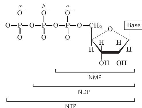
FIGURE 8-36 Nucleoside phosphates. General structure of the nucleoside 5'-mono-, di-, and triphosphates (NMPs, NDPs, and NTPs) and
