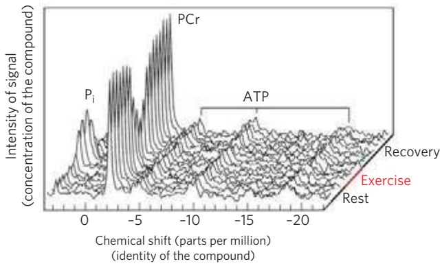
FIGURE 23-18 Phosphocreatine buffers ATP concentration during exercise. A “stack plot” of magnetic resonance spectra (of 31 P) showing inorganic phosphate (P i ), phosphocreatine (PCr), and ATP (each of its three phosphates giving a signal). The series of plots represents the passage of time, from a period of rest to one of exercise, and then of recovery. Note that the ATP signal hardly changes during exercise, kept high by continued respiration and by the reservoir of phosphocreatine, which diminishes during exercise. During recovery, when ATP production by catabolism is greater than ATP utilization by the (now resting) muscle, the phosphocreatine reservoir is refilled.
