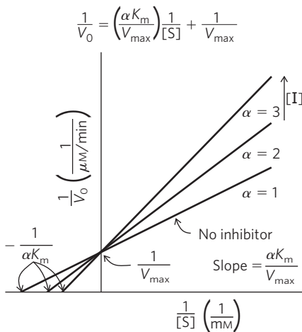
FIGURE 1 Competitive inhibition.
