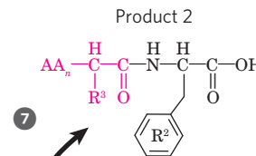
Enzyme-product 2 complex
