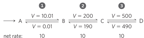
FIGURE 15-6 Near-equilibrium and nonequilibrium steps in a metabolic pathway. Steps 2 and 3 of this pathway are near equilibrium in the cell; for each step, the rate ( V ) of the forward reaction is only slightly greater than the reverse rate, so the net forward rate (10) is relatively low and the free-energy change, \Delta G , is close to zero. An increase in [C] or [D] can reverse the direction of these steps. Step 1 is maintained in the cell far from equilibrium; its forward rate greatly exceeds its reverse rate. The net rate of step 1 (10) is much larger than the reverse rate (0.01) and is identical to the net rates of steps 2 and 3 when the pathway is operating in the steady state. Step 1 has a large, negative \Delta G .
