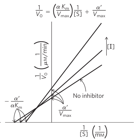
FIGURE 3 Mixed inhibition.
