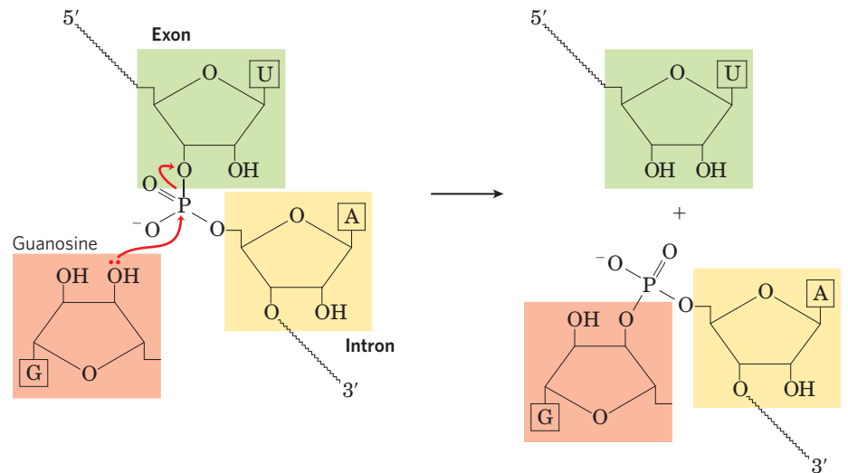
FIGURE 26-13 Transesterification reaction.
