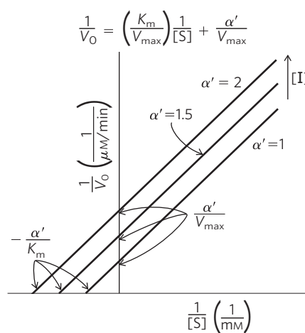
FIGURE 2 Uncompetitive inhibition.
